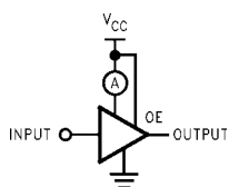
FIGURE 1. AC Test Circuit
