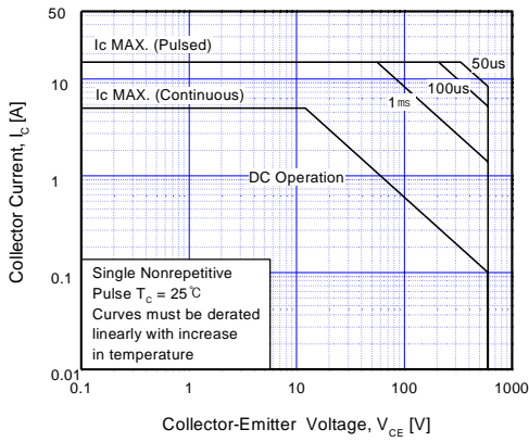
Fig 15. SOA Characteristic
