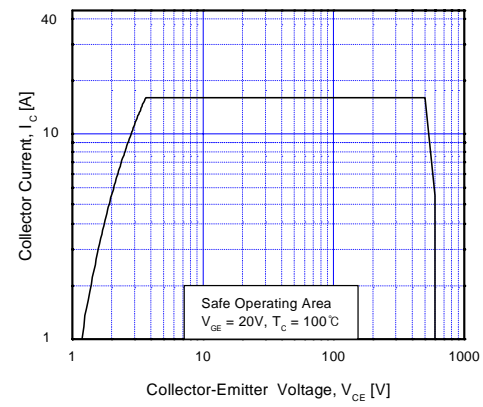
Fig 16. Turn-Off SOA Characteristics
