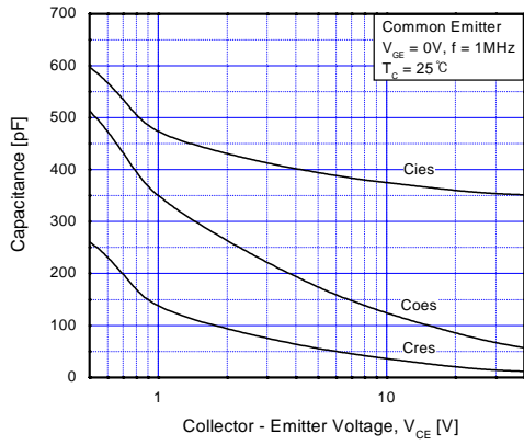
Fig 7. Capacitance Characteristics
