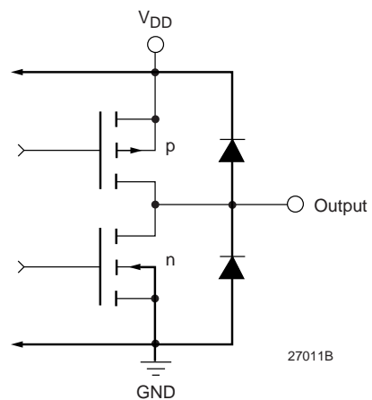
Figure 4. Equivalent Digital Output Circuit
