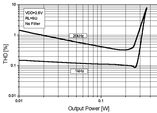
Figure 3. THD+N versus output power
