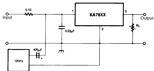
Figure 7. Ripple Rejection
