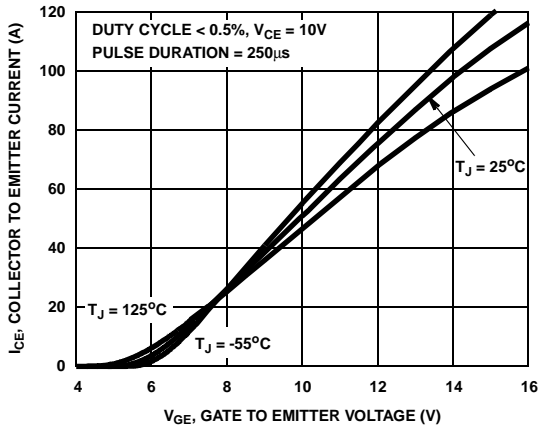
Figure 13. Transfer Characteristic
