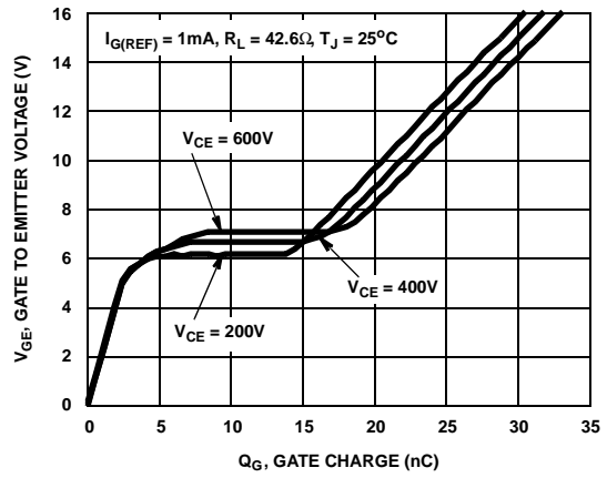
Figure 14. Gate Charge
