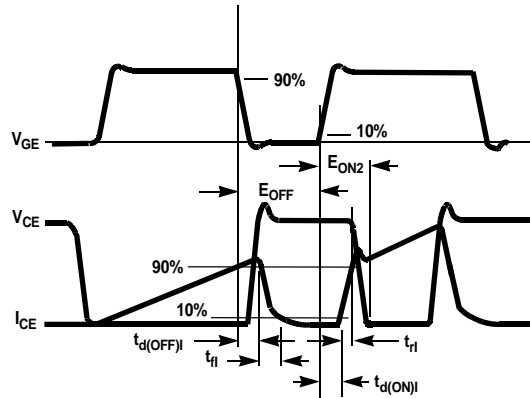
Figure 27. Switching Test Waveforms
