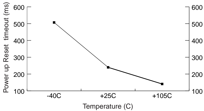
Power up Reset Timeout Vs. Temperature
