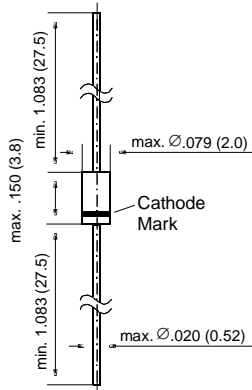
DO-35
