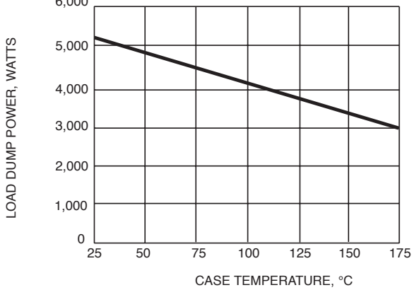
FIG. 5 - LOAD DUMP POWER CHARACTERISTICS (10ms EXPONENTIAL WAVEFORM)
