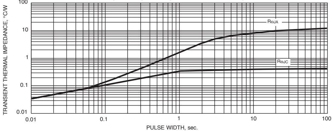
FIG. 7 - TYPICAL TRANSIENT THERMAL IMPEDANCE
