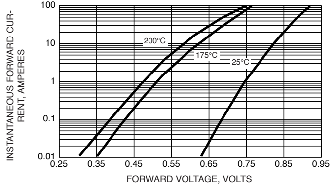
FIG. 2 - TYPICAL INSTANTANEOUS FORWARD CHARACTERISTICS
