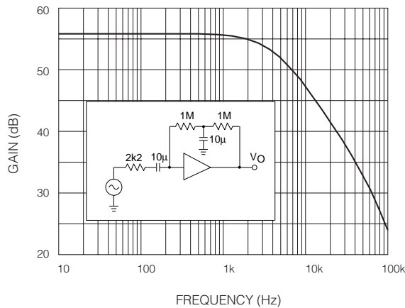
Fig. 7 Open Loop Voltage Gain
