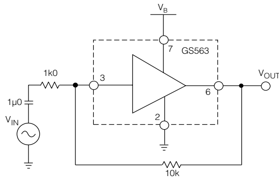
Fig. 4 Characterization Circuit
