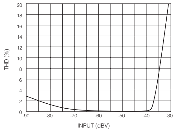
Fig. 6 THD vs Input Level
