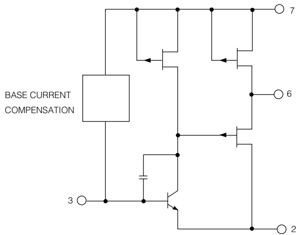
Fig. 2 Functional Schematic
