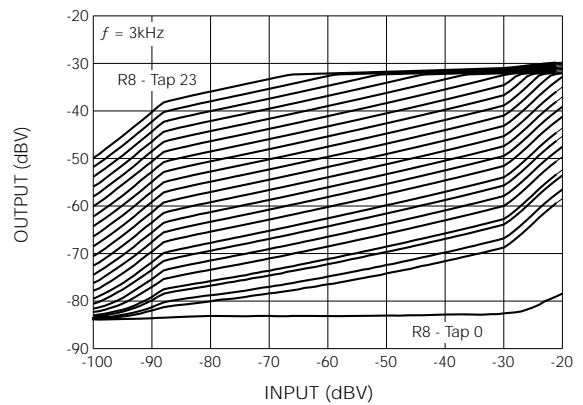
Fig. 10 System Volume Control (Tap 0 - 0kΩ, Tap 23 - 92kΩ)
