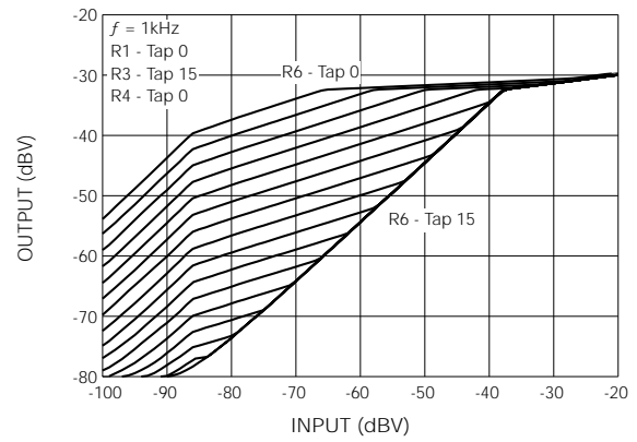
Fig. 6 Low Frequency Gain Control (Tap 0 - 185kΩ, Tap 15 - 0kΩ)
