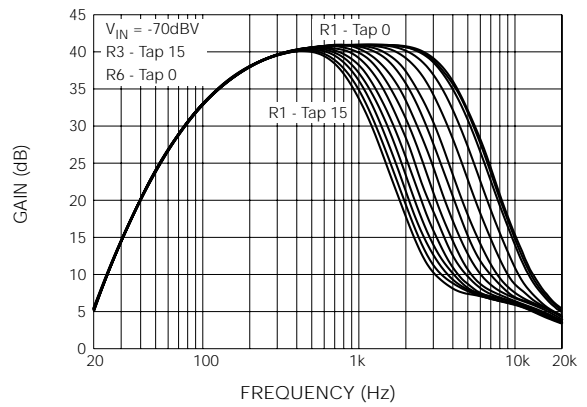
Fig. 12 SVF Crossover Frequency - Low Pass (Tap 0 - 0kΩ, Tap 15 - 64kΩ)
