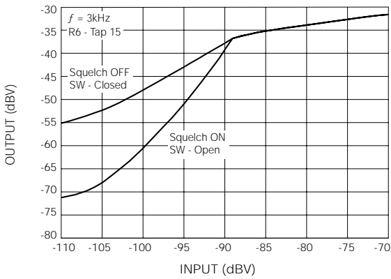
Fig. 11 Low Level Squelch Control
