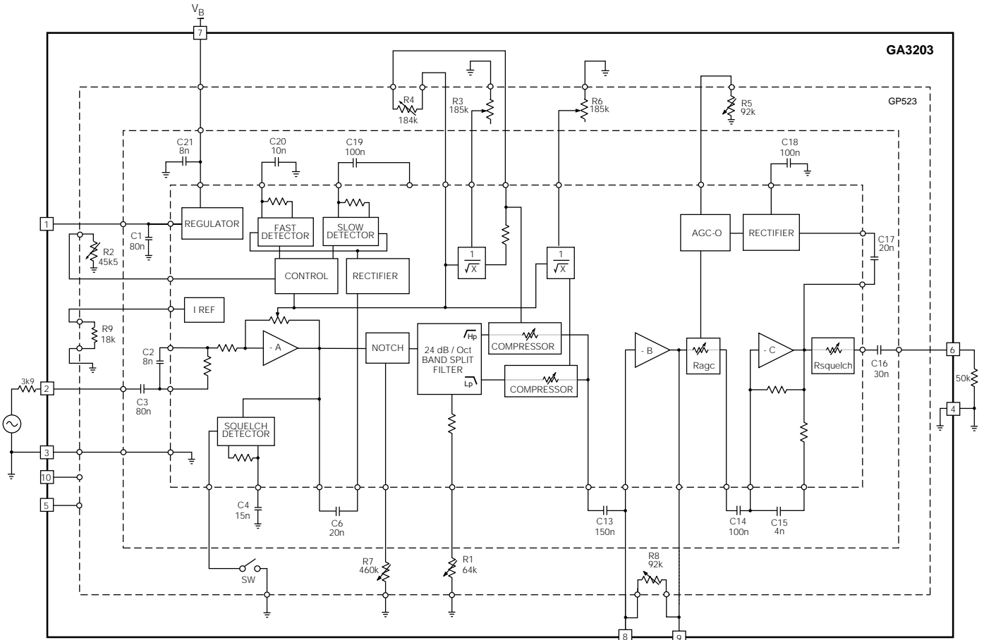
Fig. 1 Test Circuit
