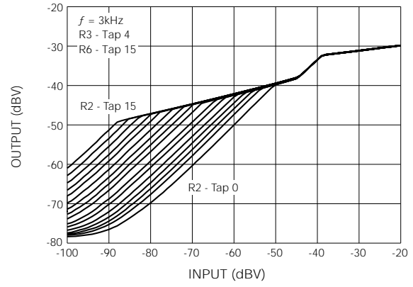
Fig. 8 AGC-I Threshold Control (Tap 0 - 0kΩ, Tap 15 - 45.5kΩ)
