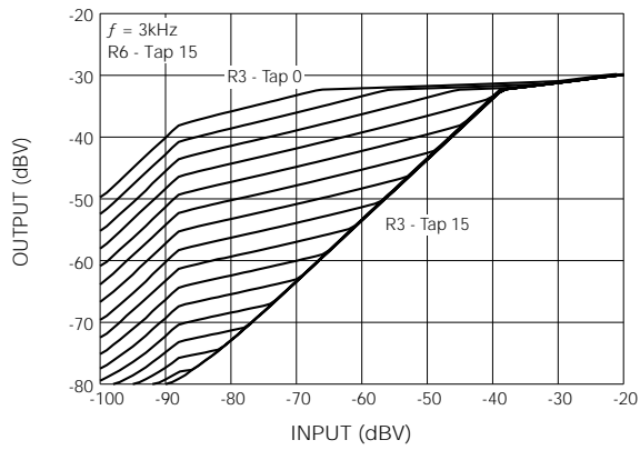
Fig. 5 High Frequency Gain Control (Tap 0 - 185kΩ, Tap 15 - 0kΩ)
