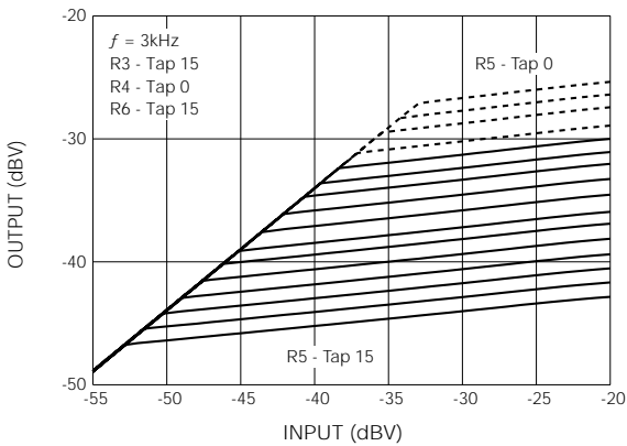
Fig. 9 AGC-O Threshold Control (Tap 0 - 7.3kΩ, Tap 15 - 92kΩ)
