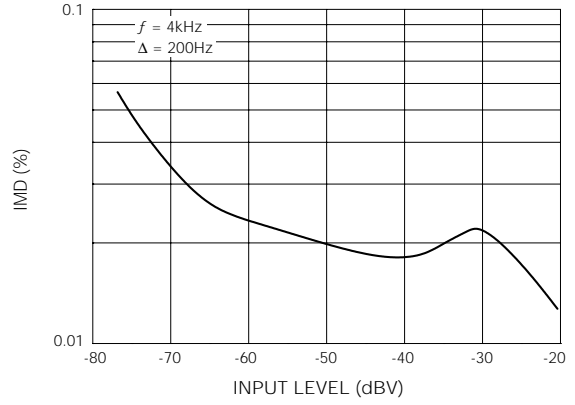
Fig. 18 Intermodulation Distortion (CCIF) vs. Input Level
