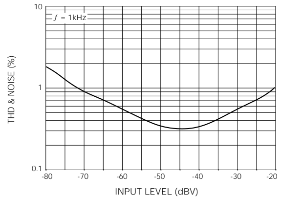
Fig. 16 THD and Noise vs. Input Level
