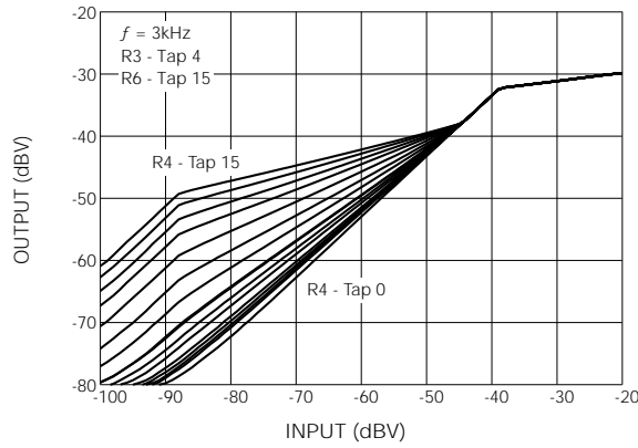
Fig. 7 High Frequency Compression Ratio Control (Tap 0 - 0kΩ, Tap 15 - 184kΩ)
