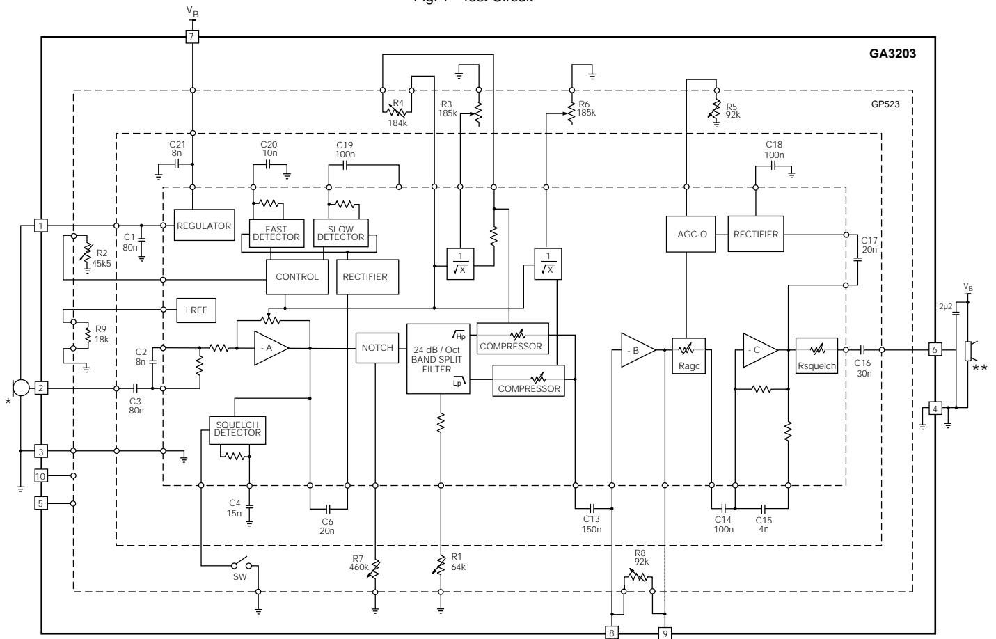
Fig. 1 Test Circuit
