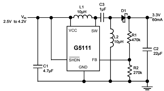
L1, L2: MURATA LQH3C100K24 D1: MOTOROLA MBR0520
