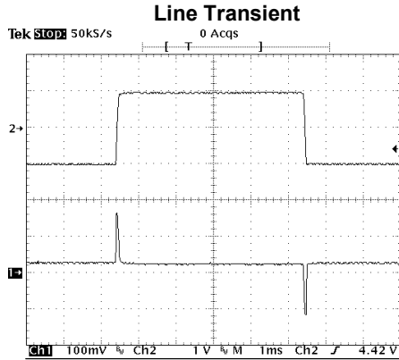
Ch1: Vout (offset=3.30V) Ch2: Vin (offset=5.0V) Iout=100mA
