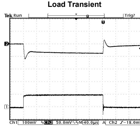
Ch1: Iout (400mA/div) Ch2: Vout (offset=3.30V)
