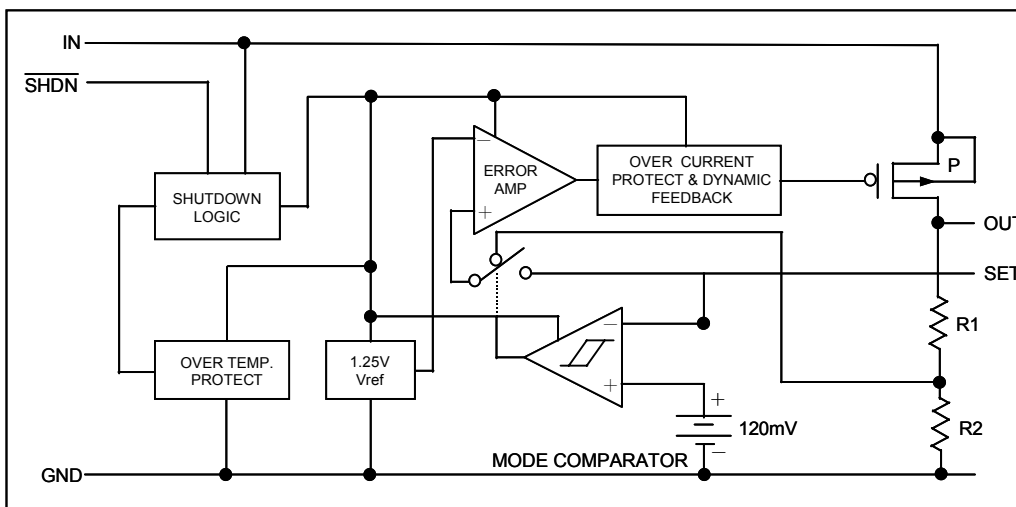
Figure 1. Functional Diagram
