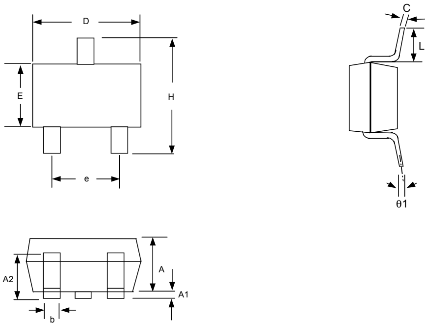
SOT-23 (T7) Package
