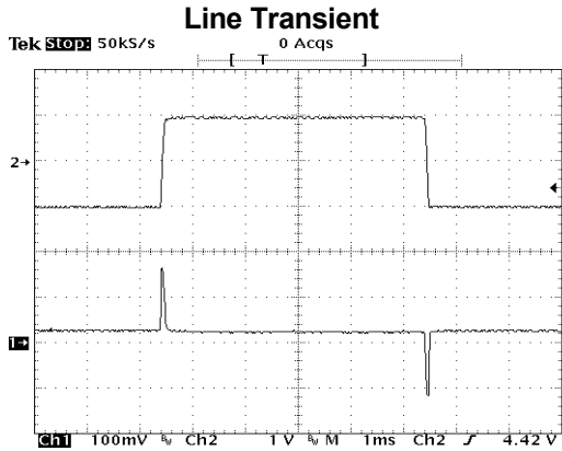
Ch1: Vout (offset=3.70V) Ch2: Vin (offset=5.0V) Iout=100mA
