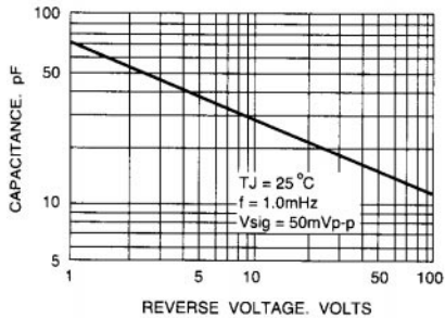
FIG. 5 - TYPICAL JUNCTION CHARACTERISTICS
