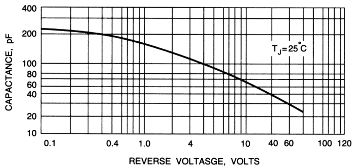
Fig. 4 - TYPICAL JUNCTION CAPACITANCE
