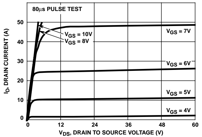
FIGURE 5. OUTPUT CHARACTERISTICS
