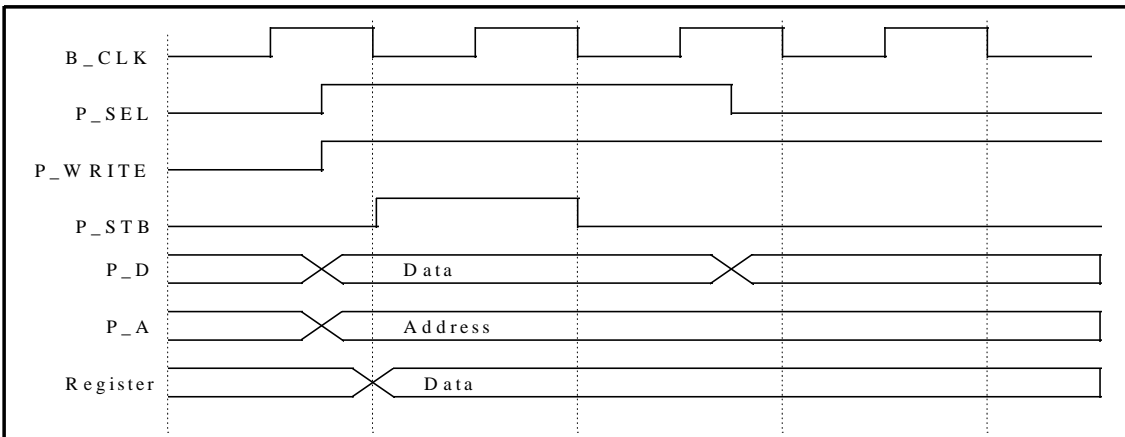
Figure 3. APB Write
