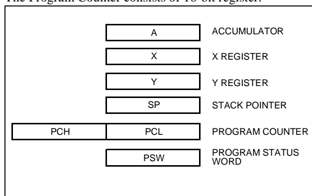
Figure 8-1 Configuration of Registers
