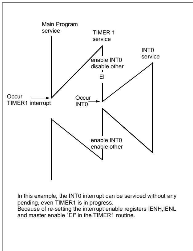
Figure 19-7 Execution of Multi Interrupt
