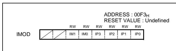
Figure 19-1 Interrupt Mode Register
