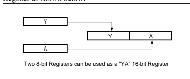
Figure 8-2 Configuration of YA 16-bit Register
