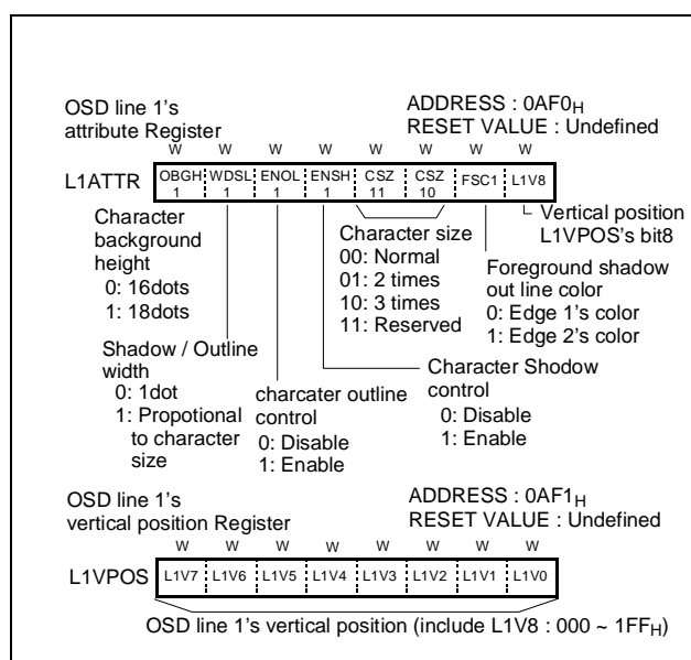
Figure 17-6 OSD Registers - 3
