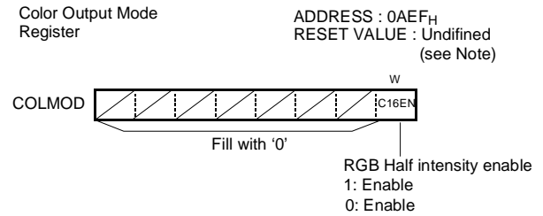
Figure 17-10 OSD Register - 7
