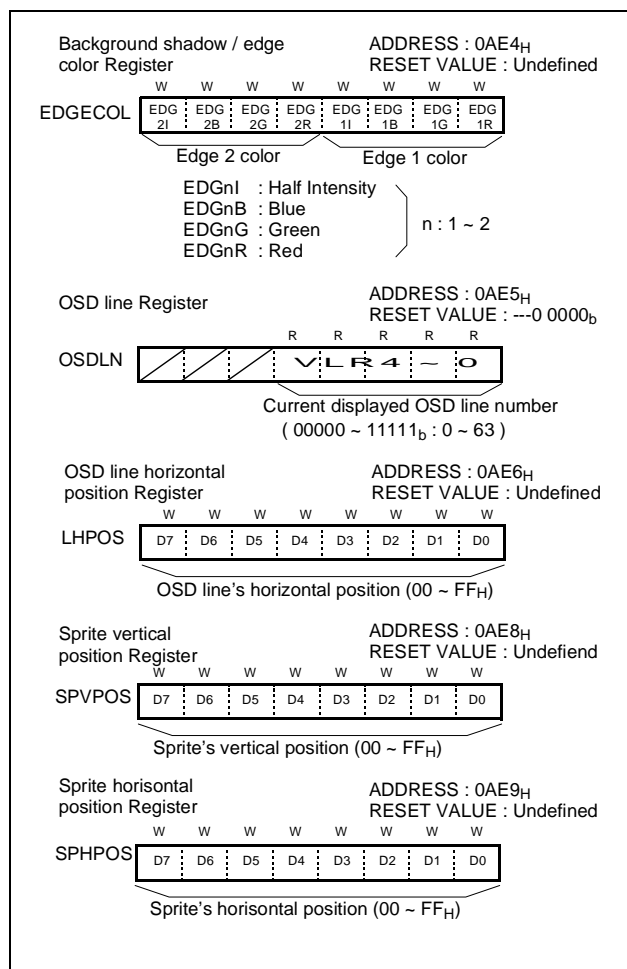
Figure 17-6 OSD Registers - 3
