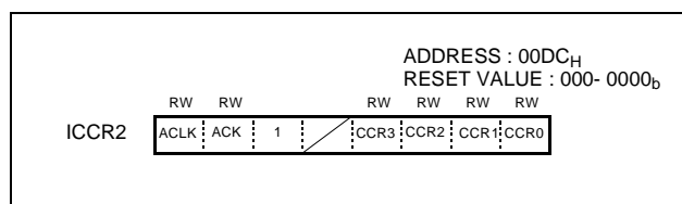
Figure 18-6 I 2 C control Register 2
