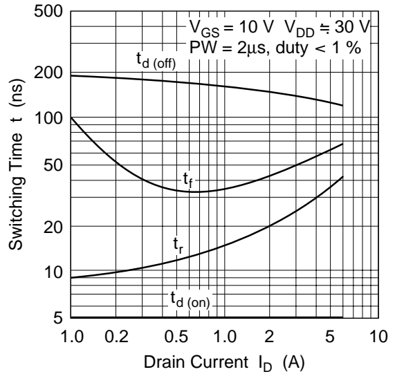
Switching Characteristics
