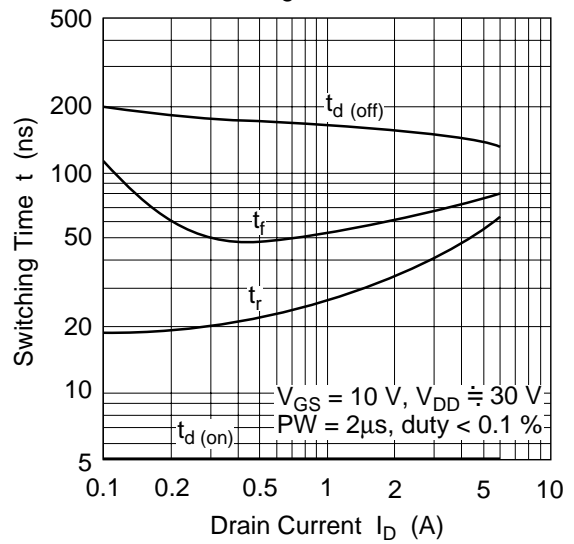
Switching Characteristics
