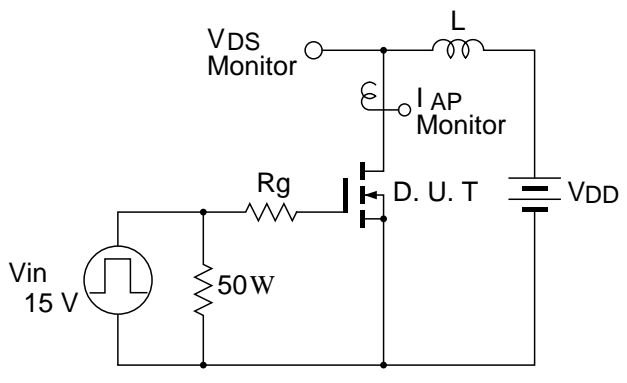
Avalanche Test Circuit
