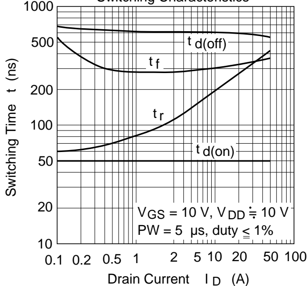
Switching Characteristics
