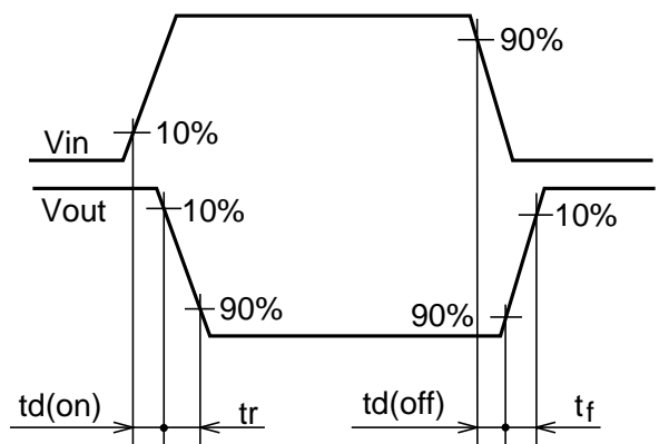
Waveform
