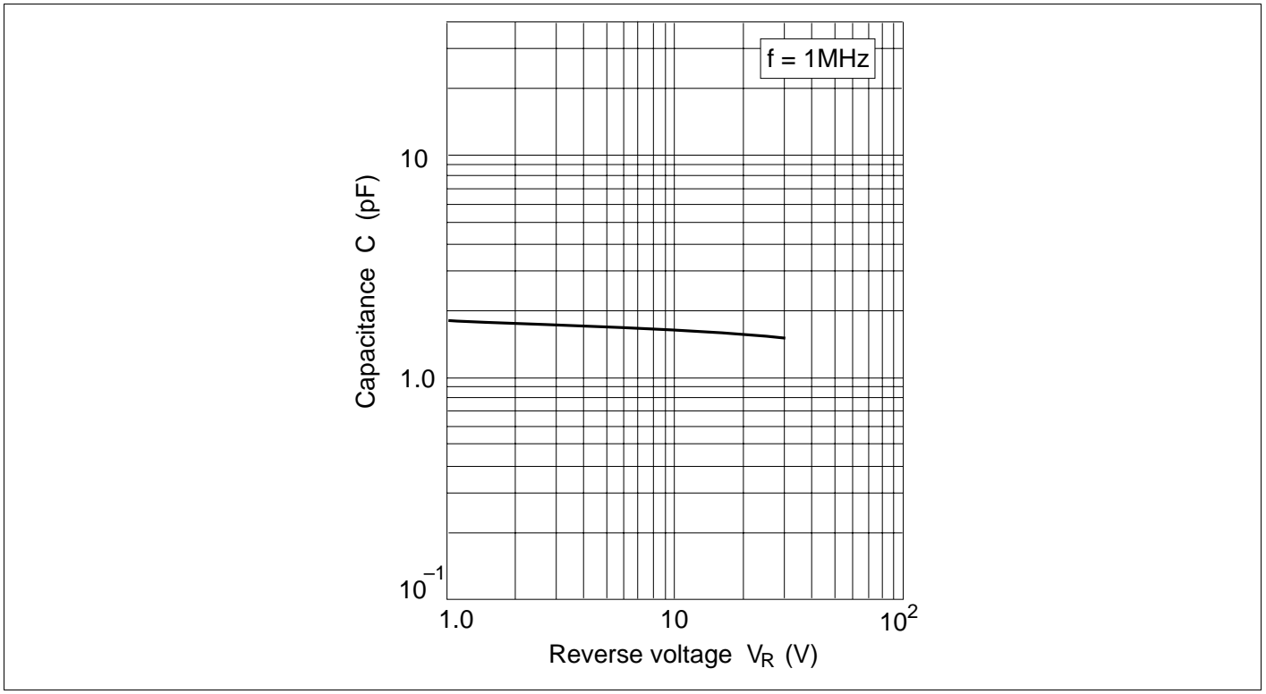
Fig.3 Capacitance Vs. Reverse voltage
