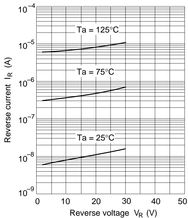
Fig.2 Reverse current Vs. Reverse voltage
