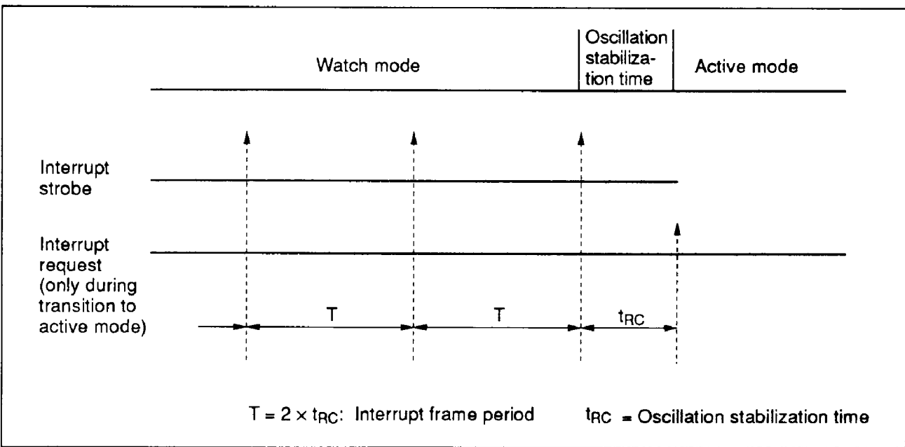
Figure 14 Interrupt Frame
