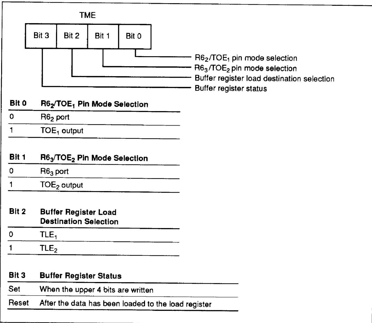
Figure 31 Timer Mode Register E
