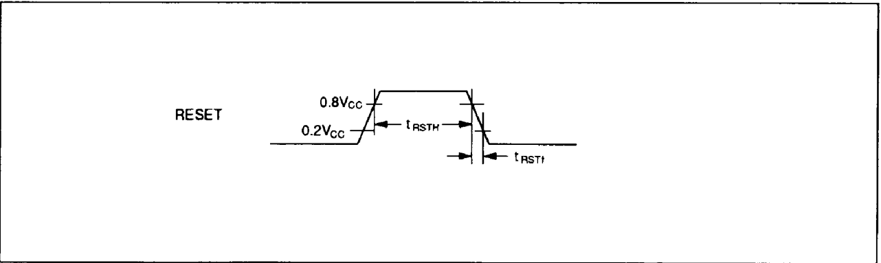
Figure 50 Reset Timing
