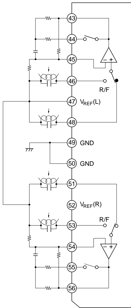
Figure 3 Application Circuit
