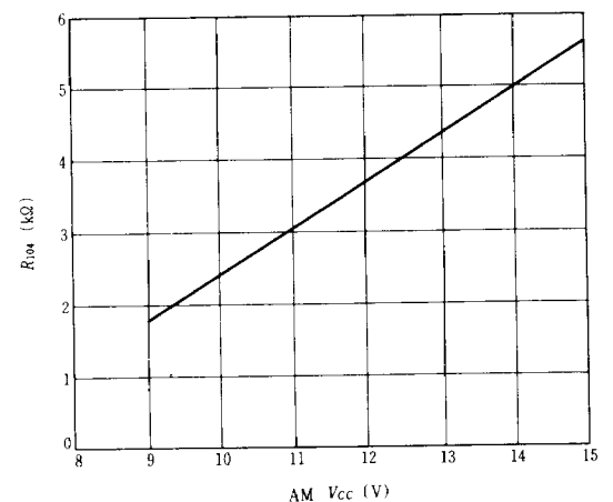
■ R 104 (Resistor of Pin-15) vs. AM V CC
