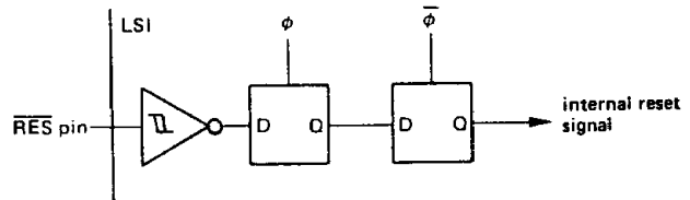
Figure 33 RES circuit
