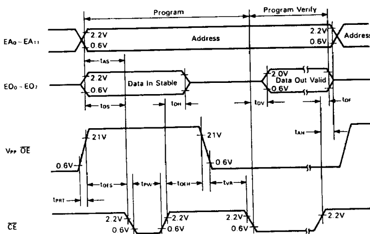
Figure 12 EPROM Programming Timing
