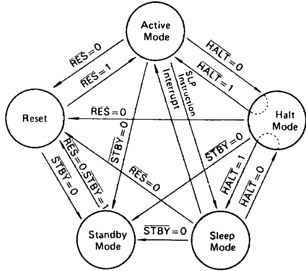
Figure 28 CPU Operation Mode Transition
