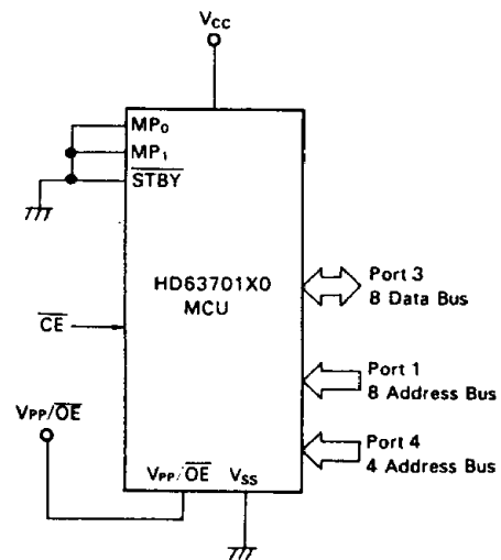
Figure 19 EPROM Mode
