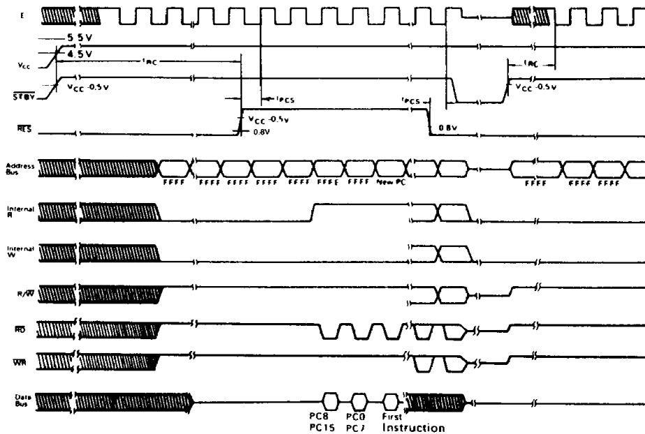
Figure 11 Reset Timing
