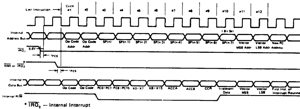
Figure 10 Interrupt Sequence
