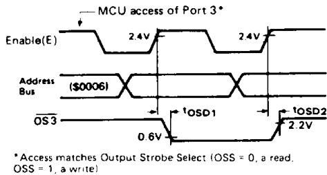
Figure 5 Port 3 Output Strobe Timing (Single Chip Mode)
