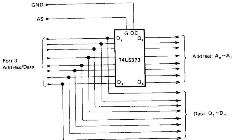
Figure 19 Latch Connection
