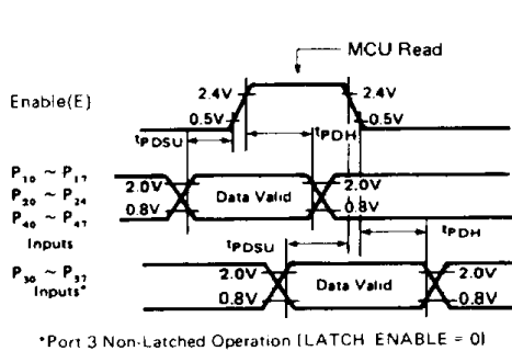
Figure 3 Data Set-up and Hold Times (MCU Read)
