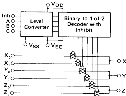
Figure 15 HD14053B Multiplexers/Demultiplexers
