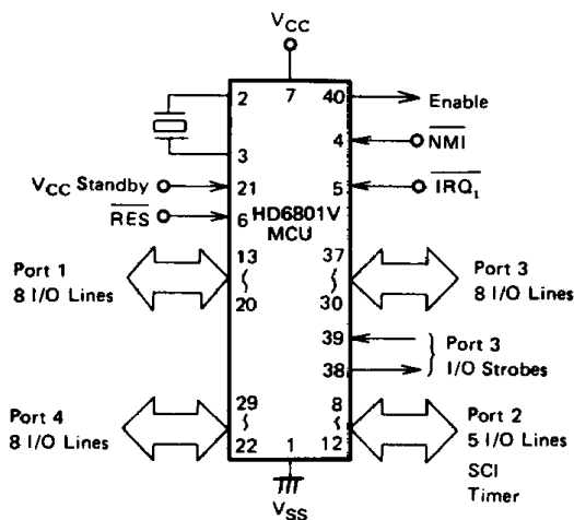
Figure 16 HD6801V MCU Single-Chip Mode
