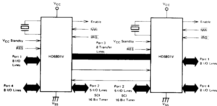
Figure 25 HD6801V MCU Single-Chip Dual Processor Configuration
