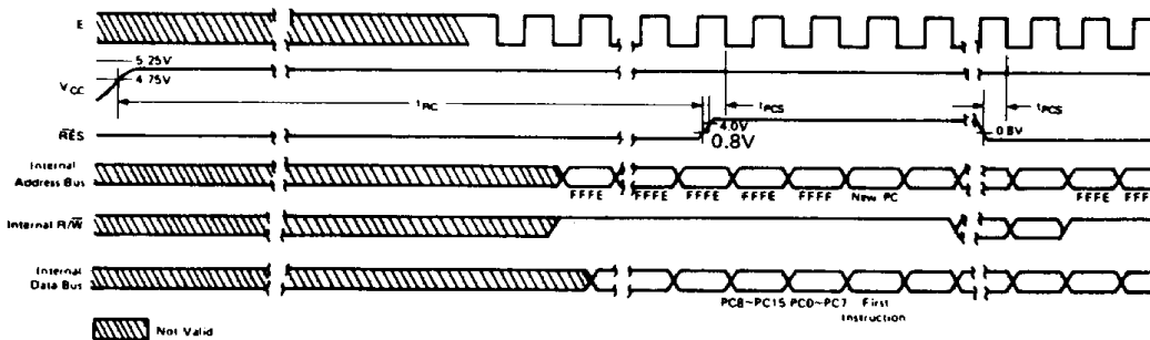
Figure 11 Reset Timing
