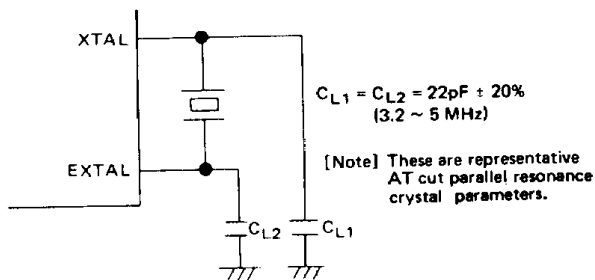
Figure 12 Crystal Interface
