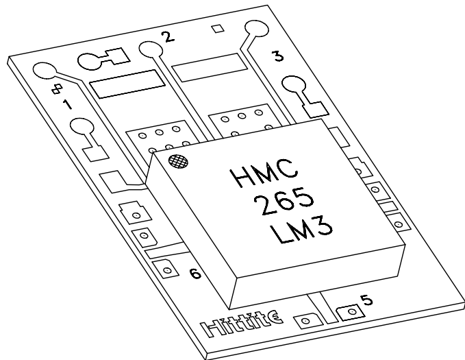
LM3 package mounted to evaluation PCB
