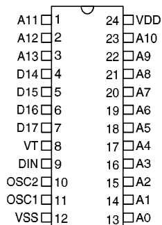
HT644L – 24 SOP/SDIP
