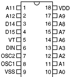
HT692 - 18 DIP
