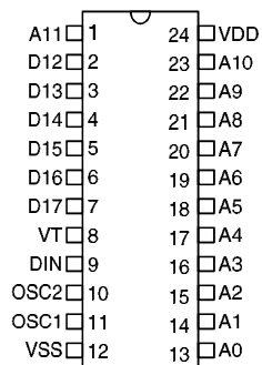
HT656 – 24 SOP/SDIP
