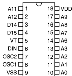
HT682L – 18 DIP
