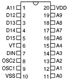
HT604L – 20 DIP/SOP
