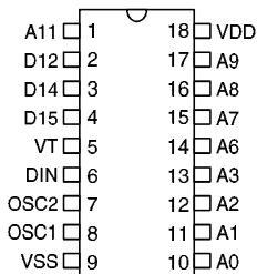
HT683L – 18 DIP
