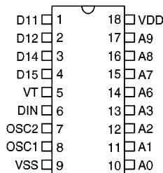
HT684L – 18 DIP
