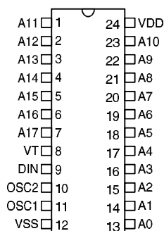
HT651 – 24 SOP/SDIP
