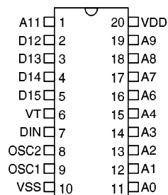
HT614 – 20 DIP/SOP
