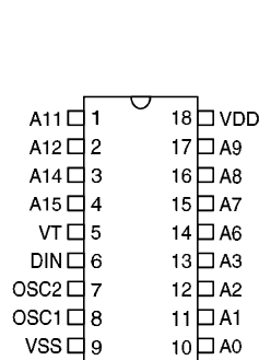
HT691 – 18 DIP
