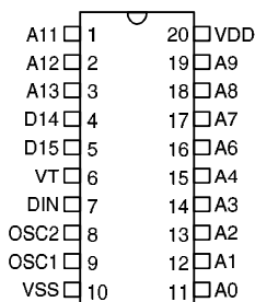
HT612 – 20 DIP/SOP
