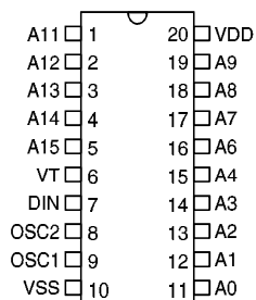
HT611 – 20 DIP/SOP
