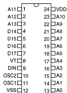
HT654 – 24 SOP/SDIP
