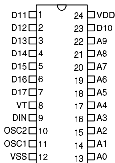
HT658 – 24 SOP/SDIP
