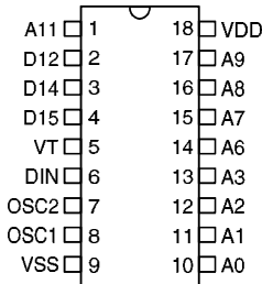
HT693 - 18 DIP
