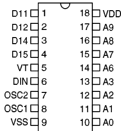
HT694 - 18 DIP
