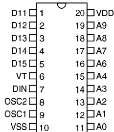
HT605L – 20 DIP/SOP
