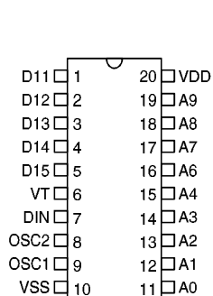
HT615 – 20 DIP/SOP
