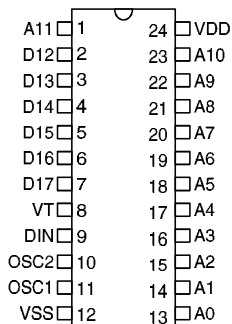
HT646L – 24 SOP/SDIP
