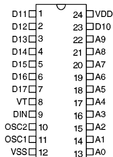
HT648L – 24 SOP/SDIP
