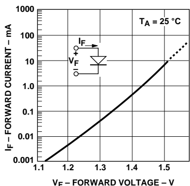
Figure 4. Typical Input Diode Forward Characteristic.
