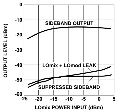
Figure 14. Modulator + Mixer SSB Output Levels vs. LMod Power Input.
