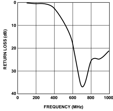
Figure 12. HPMX-3002 Output Return Loss vs. Frequency.
