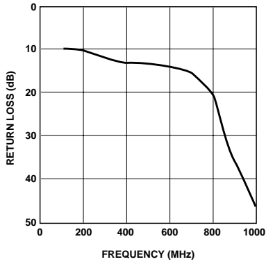
Figure 11. HPMX-3002 Input Return Loss vs. Frequency.
