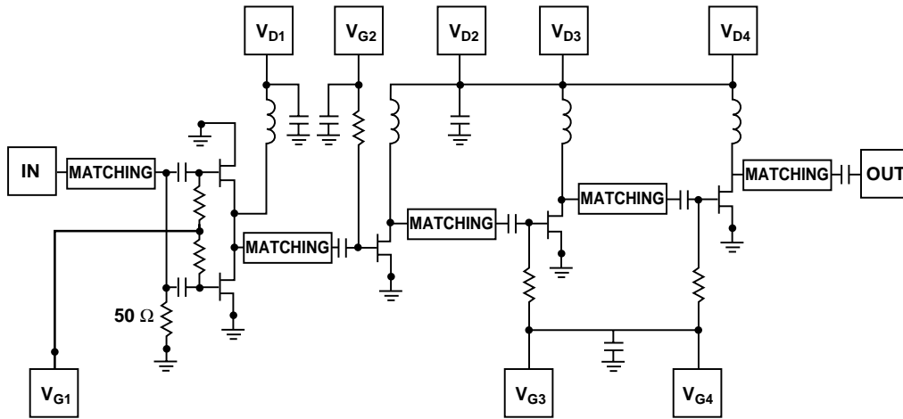
Figure 1. HMMC-5040 Simplified Schematic Diagram.
