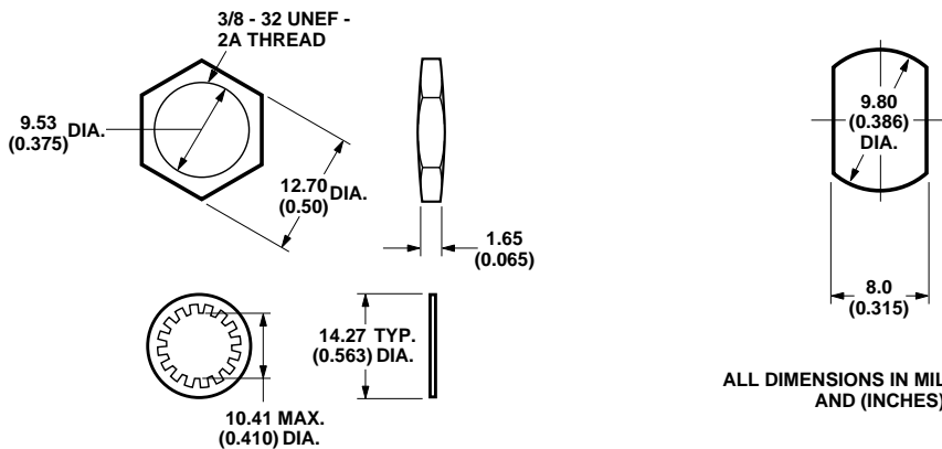
INTERNAL TOOTH LOCK WASHER
