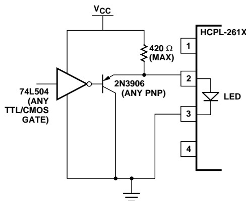
Figure 22. TTL Interface Circuit for the HCPL-261A/-261N Families.
