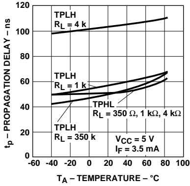
Figure 11. Typical Propagation Delay vs. Temperature.
