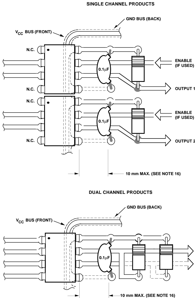
Figure 19. Recommended Printed Circuit Board Layout.
