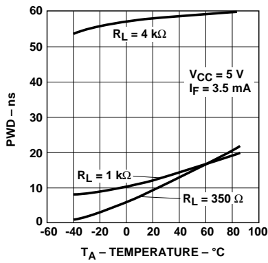
Figure 13. Typical Pulse Width Distortion vs. Temperature.
