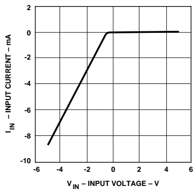
Figure 16. Typical Input Current vs. Input Voltage.
