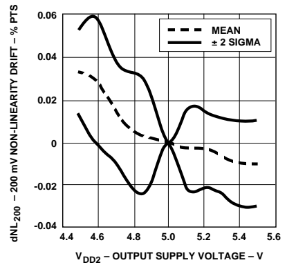
Figure 12. 200 mV Nonlinearity Drift vs. V_{DD2} ( V_{DD1} = 5 V).
