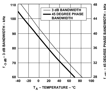
Figure 24. Typical 3 dB and 45° Bandwidths vs. Temperature.
