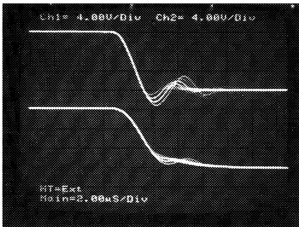
Figure 32. Application Circuit Overload Recovery Waveform.
