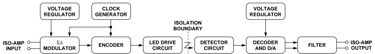
Figure 28. HCPL-7800 Block Diagram.
