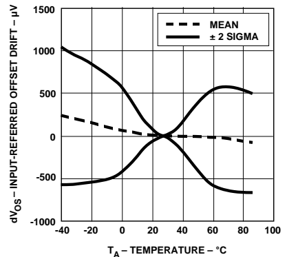
Figure 2. Input-Referred Offset Drift vs. Temperature.
