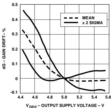
Figure 8. Gain Drift vs. V_{DD2} ( V_{DD1} = 5\text{ V} ).
