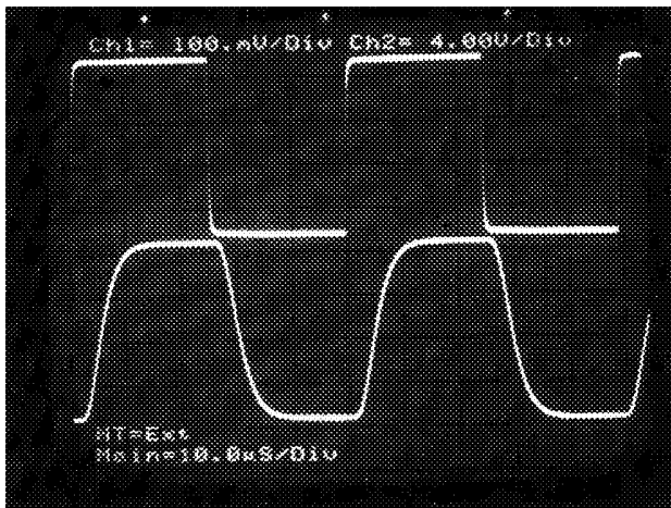
Figure 31. Application Circuit Square Wave Response.
