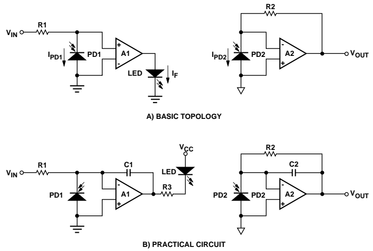
Figure 12. Basic Isolation Amplifier.
