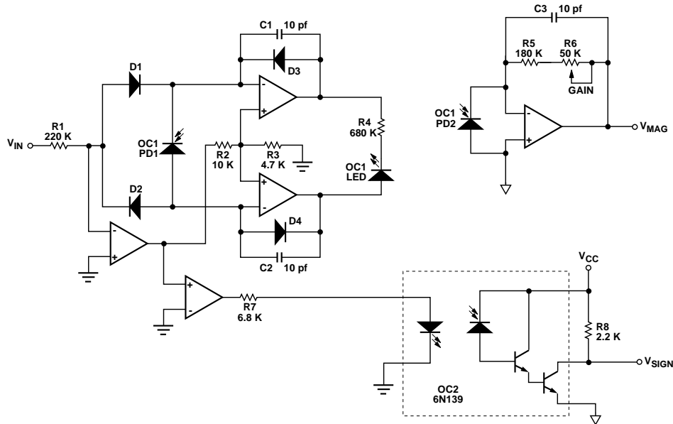
Figure 19. Magnitude/Sign Isolation Amplifier.
