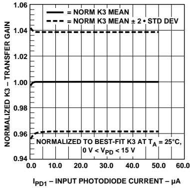
Figure 2. Normalized K3 vs. Input I_{PD} .
