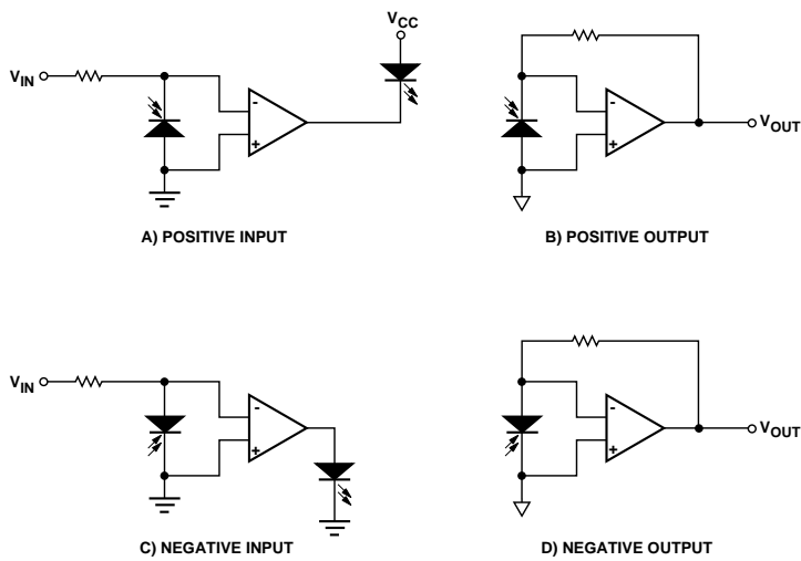
Figure 13. Unipolar Circuit Topologies.
