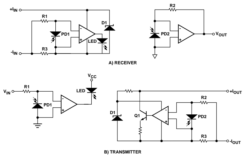
Figure 15. Loop-Powered 4-20 mA Current Loop Circuits.
