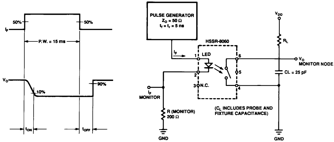
Figure 8. Switching Test Circuit for t_{ON} , t_{OFF} .
