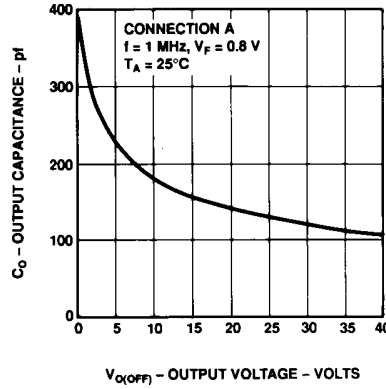
Figure 14. Typical Output Capacitance vs. Output Voltage.
