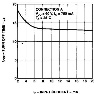
Figure 12. Typical Turn Off Time vs. Input Current.
