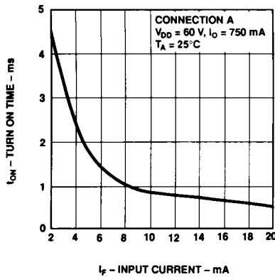
Figure 10. Typical Turn On Time vs. Input Current.
