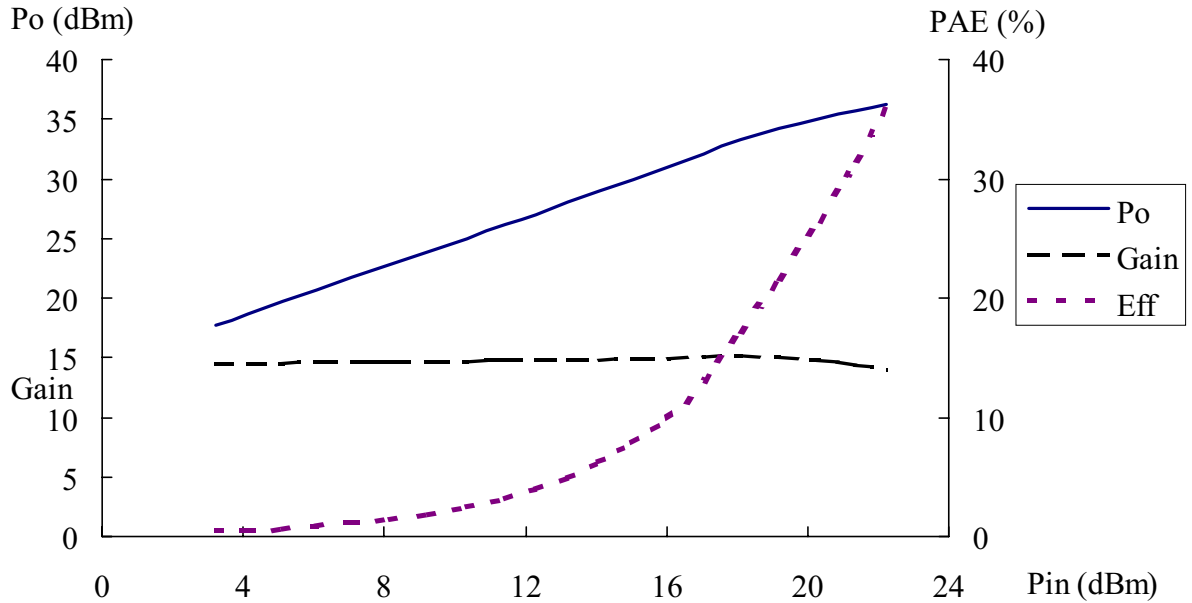
Output Power & Efficiency & Gain vs Input Power @ f=1.9 GHz, V_{ds}=10V , I_{ds} = 0.5 I_{dss}
