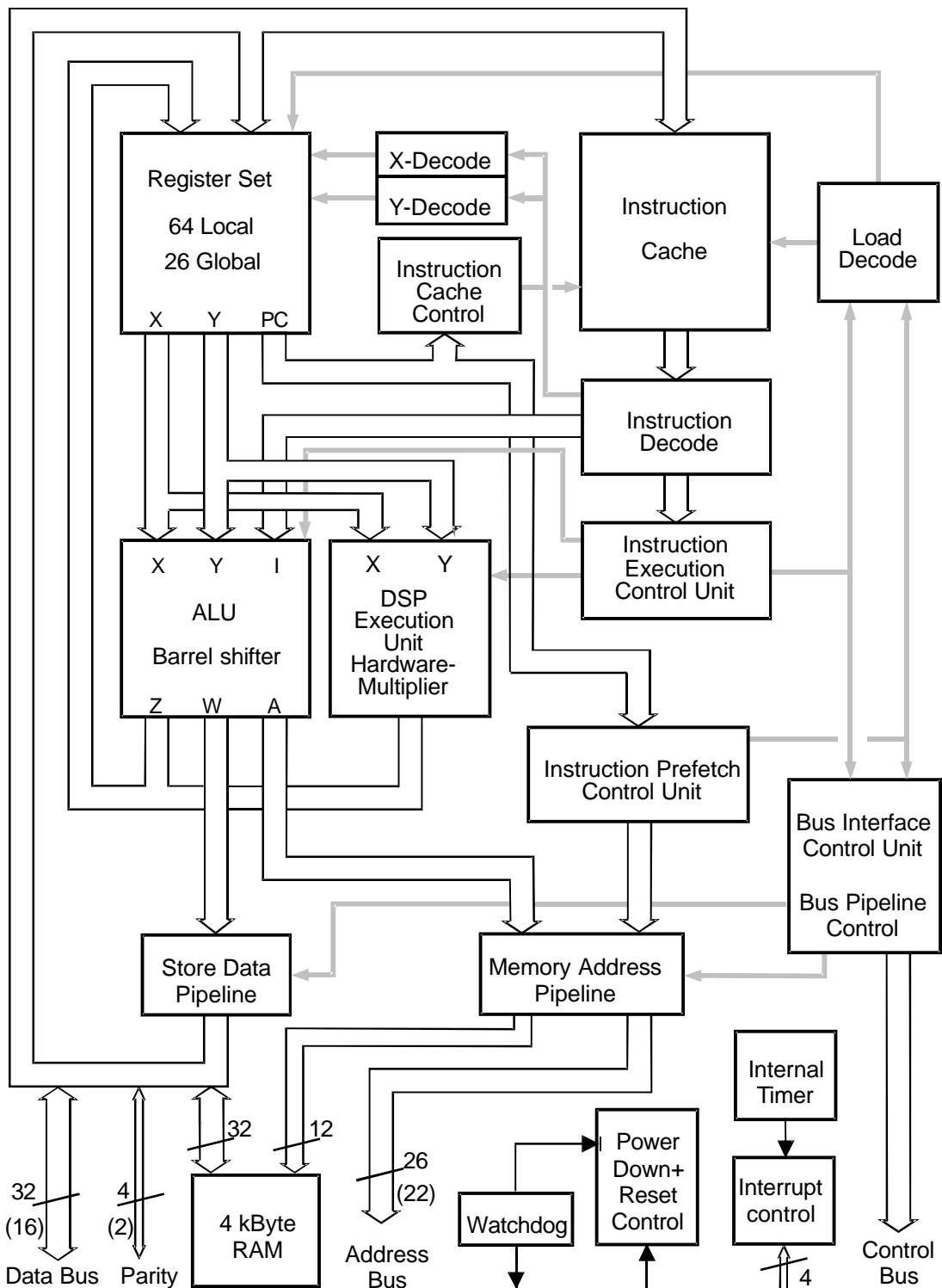
Figure 0.1: Block Diagram
