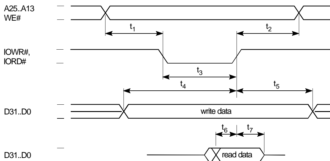
Figure 6.15: I/O Access
