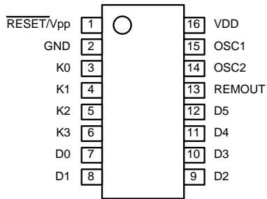
Fig 1-2 GMS34004T Pin Assignment (16PDIP)
