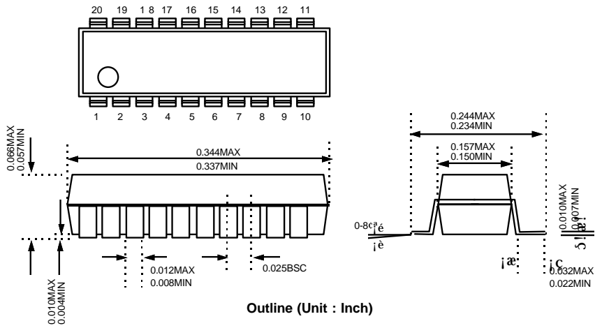
Fig 1-9 20SSOP Pin Dimension
