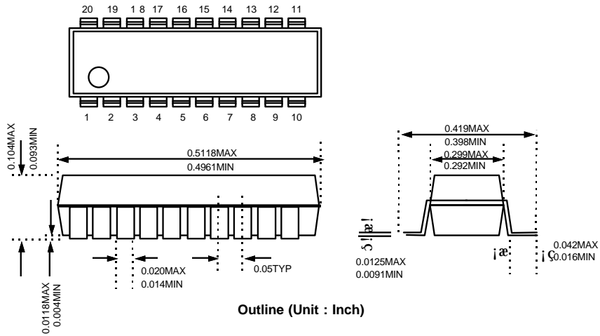
Fig 1-8 20SOP Pin Dimension
