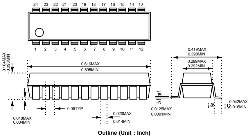
Fig 1-11 24SOP Pin Dimension
