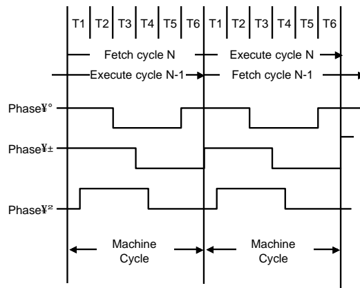
Fig. 2-3 Fundamental timing chart
