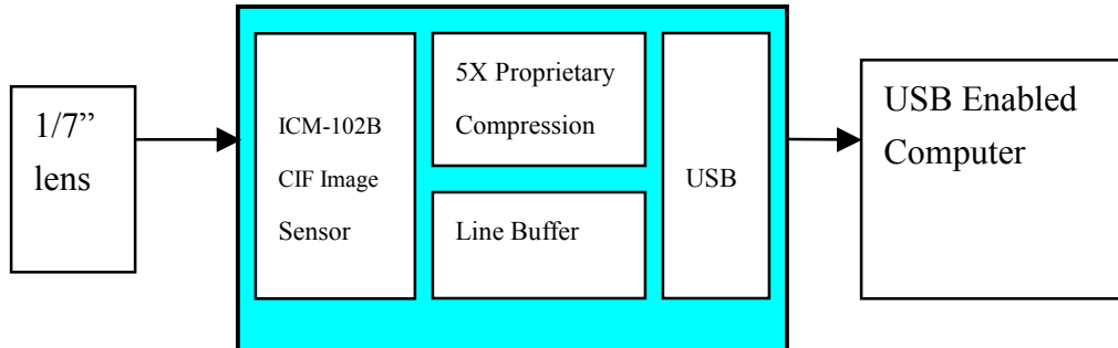
Figure 1. Block Diagram
