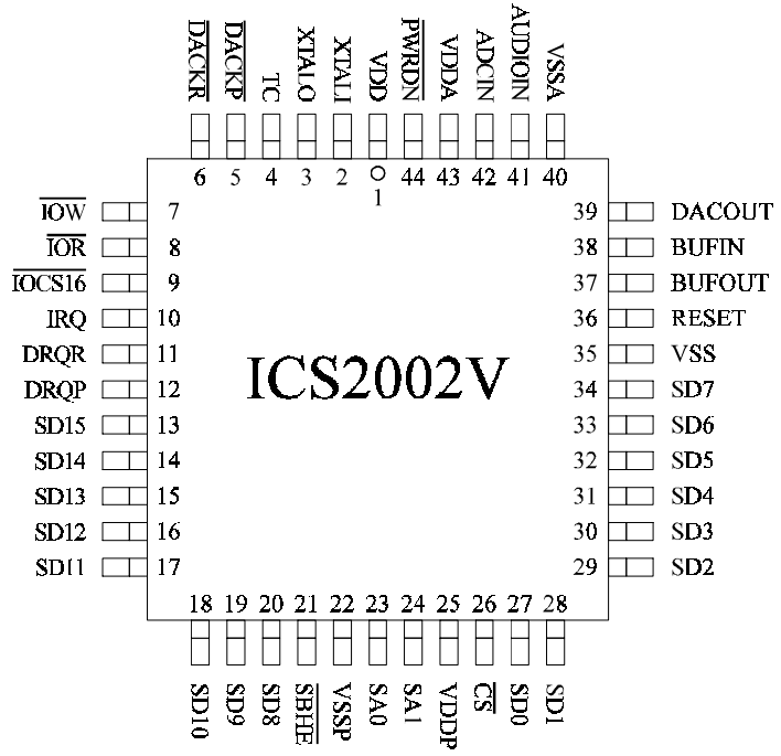
44-Pin PLCC
