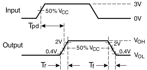
Figure 2. Voltage Waveforms Propagation Delay Times
