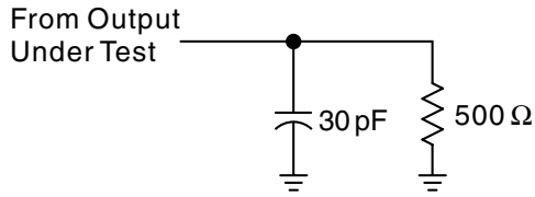
Figure 1. Load Circuit for Outputs
