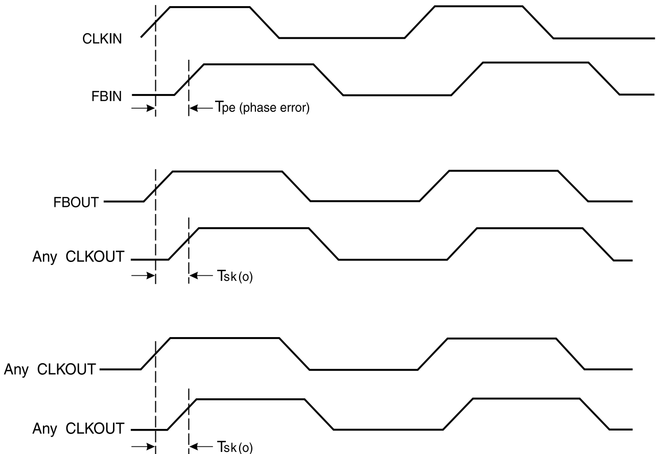
Figure 3. Phase Error and Skew Calculations
