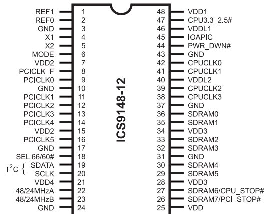
48-Pin SSOP & TSSOP
